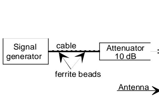
Figure D.5: Equipment set-up for the transmitting part
